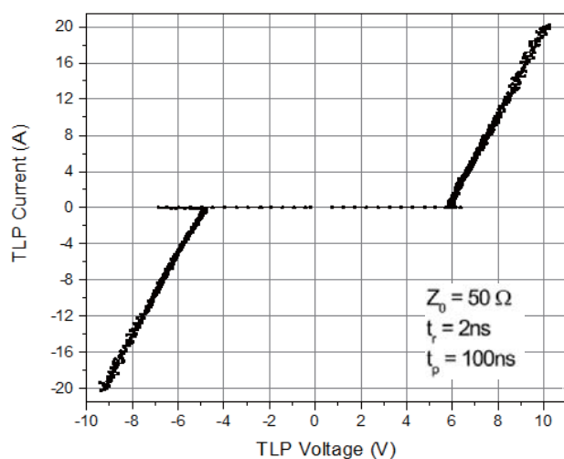
Fig5.TLP Measurement
